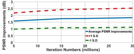
Figure 2: Average and plus/minus one standard deviation movement of SR improvement (dB) over all equirectangular panorama images as the function of the number of fine-tuning iterations. The average training time takes roughly 11 hours for 5M iterations running on NVIDIA GeForce GTX980 GPU .
