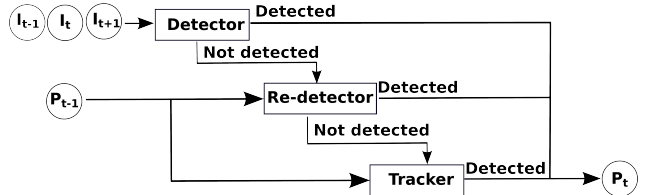
Figure 4: Flowchart of the FMO detection algorithm.
