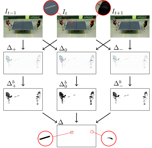
Figure 5: Detection of FMOs. Three differential images of three consecutive frames are binarized, segmented by boolean operation, and connected components are checked if they satisfy the FMO model. The two detected FMOs on this frame are the ball and the white stripe on player's t-shirt. However, only the ball passed the check and was marked as an FMO.
