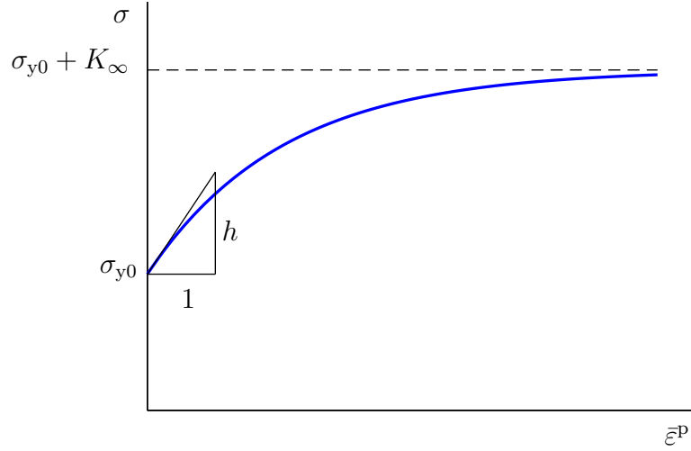
Figure 6.6: Hardening rule (6.56).
