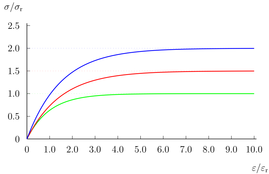
Figure 8.5: Behaviour of Maxwell's viscoelastic model in a tensile test perform with prescribed strain rates \dot{\varepsilon}_0 = \sigma_r/\eta (green line), 1.5\sigma_r/\eta (red line) and 2\sigma_r/\eta (blue line). The limiting stress is shown by dotted lines.
