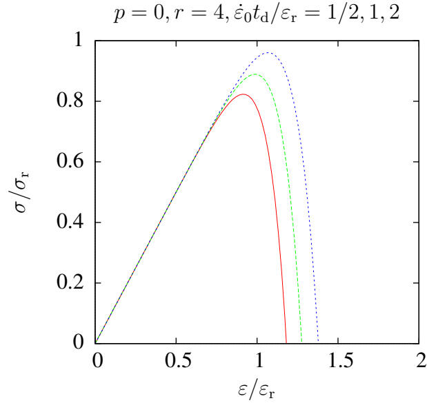
Figure 7.4: Stress-strain relation in a uniaxial constant strain-rate tensile test, \dot{\epsilon} t_d varied, i.e. either t_d varied or the loading rate \dot{\epsilon}_0 . Increasing loading rate increases the maximum stress, \dot{\epsilon}_0 t_d / \epsilon_r = 1/2 red solid, \dot{\epsilon}_0 t_d / \epsilon_r = 1 , green dashed, \dot{\epsilon}_0 t_d / \epsilon_r = 2 blue dotted curve.
